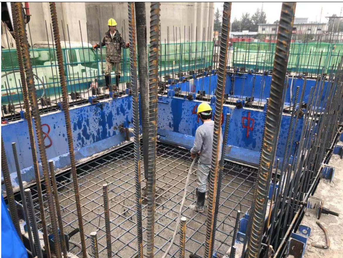
沉箱底座浇筑
